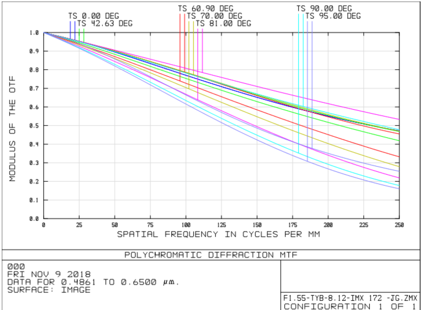
Figure 1: MTF Curves (Visible Light)
