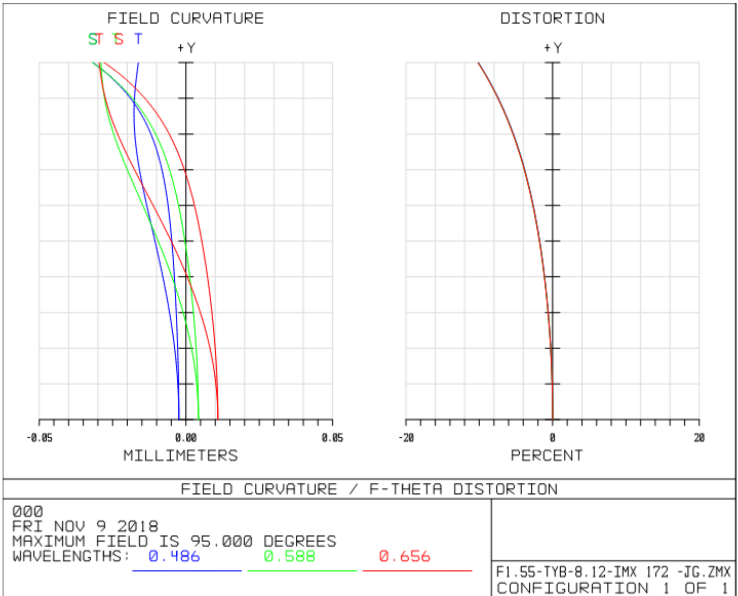
Figure 2: Field Curvature and Distortion (Visible Light)
