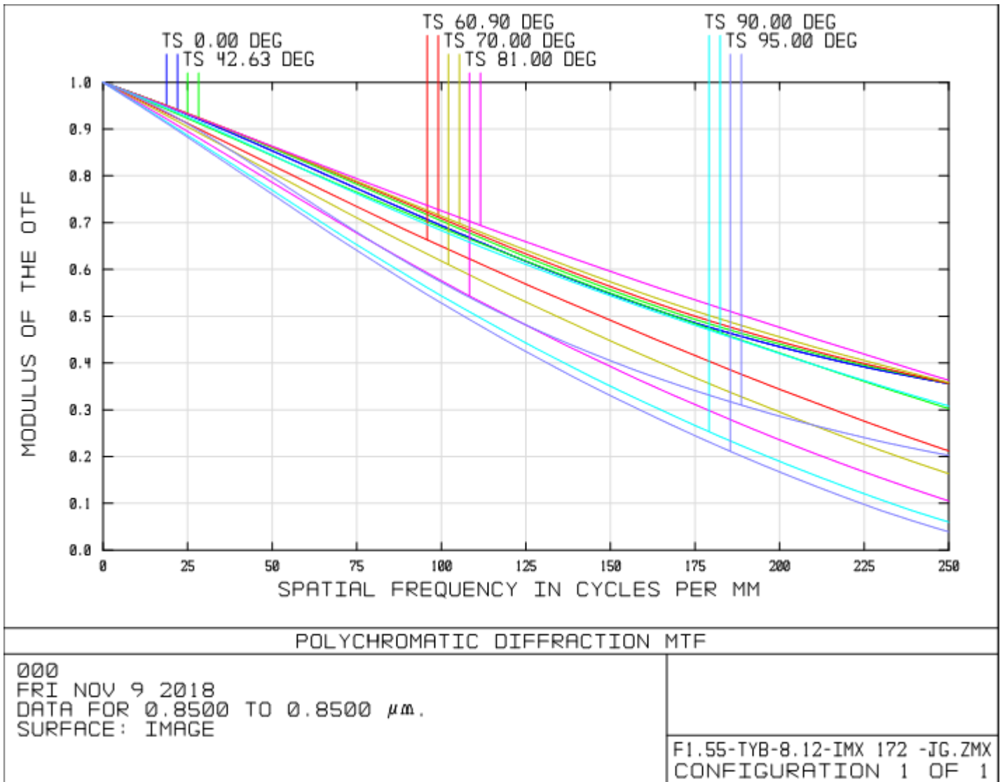
Figure 3: MTF Curves (IR)
