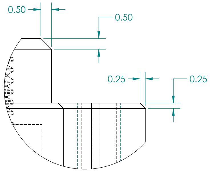
DETAIL A SCALE 10 : 1
