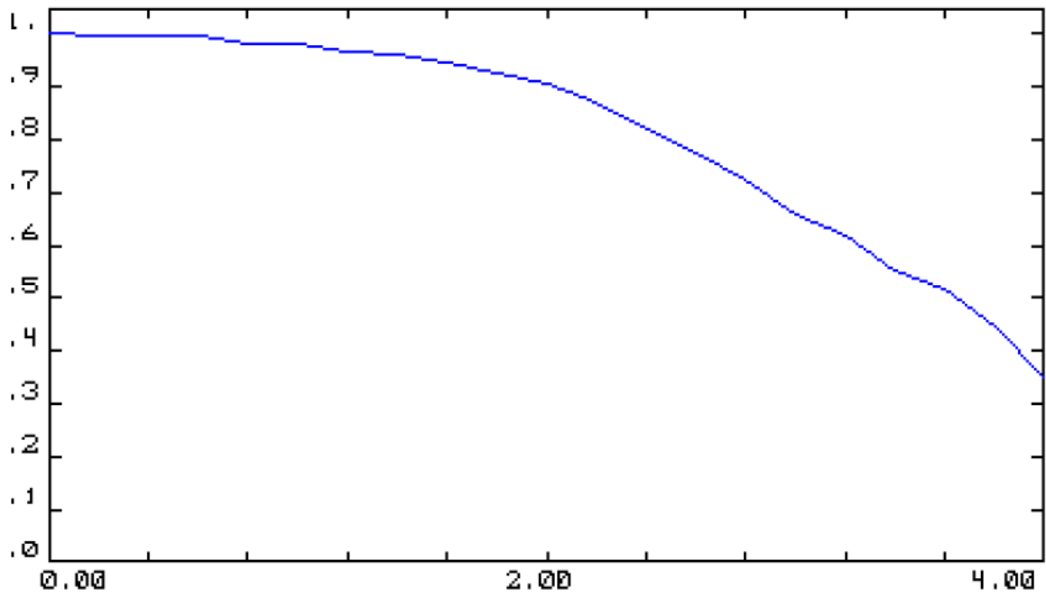
Figure 3: Relative Illumination
