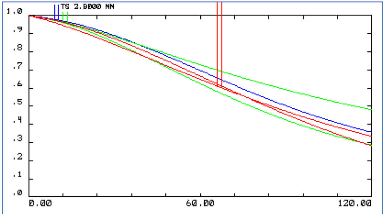
Figure 1: MTF Curves
