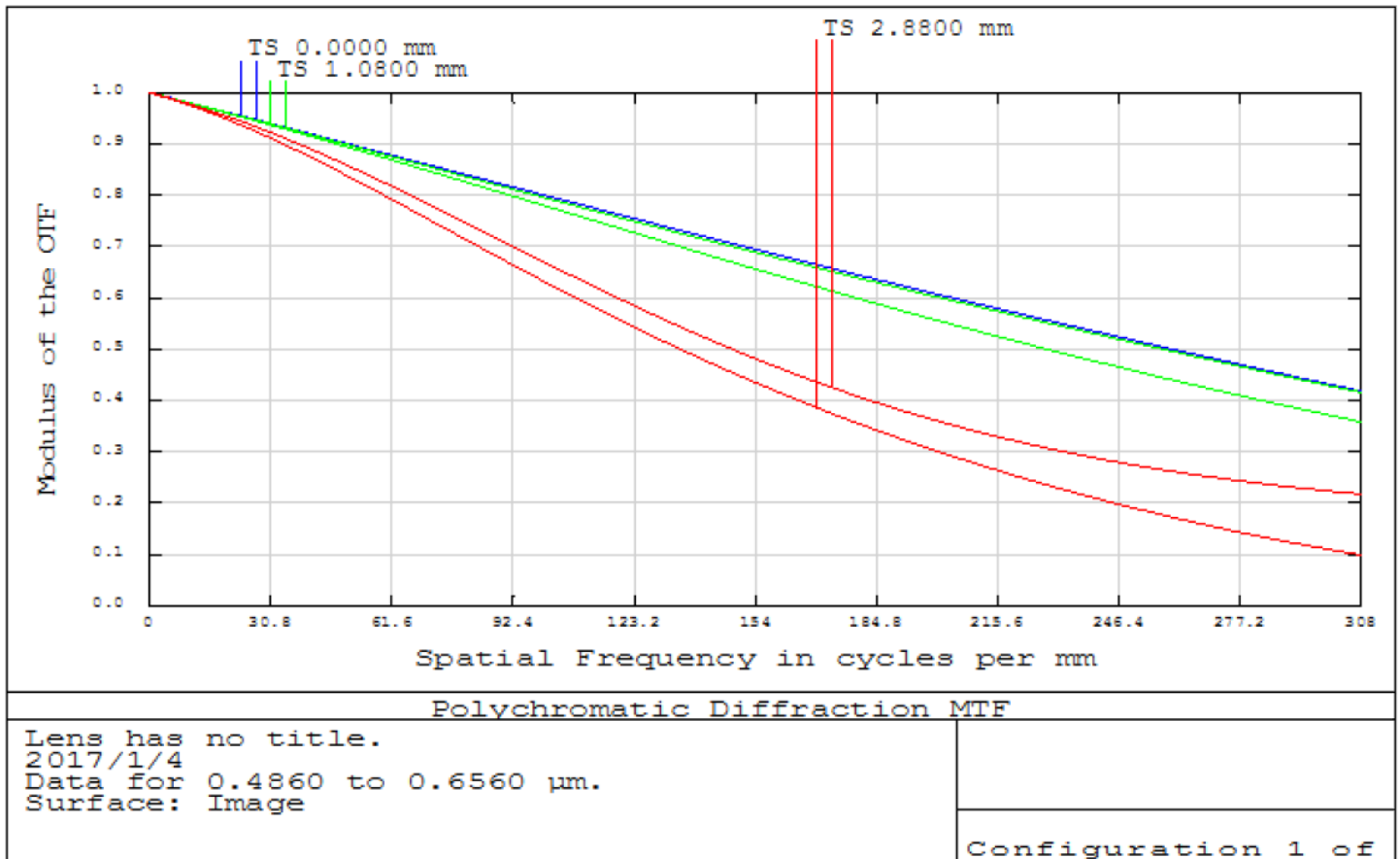
Figure 1: MTF Curves
