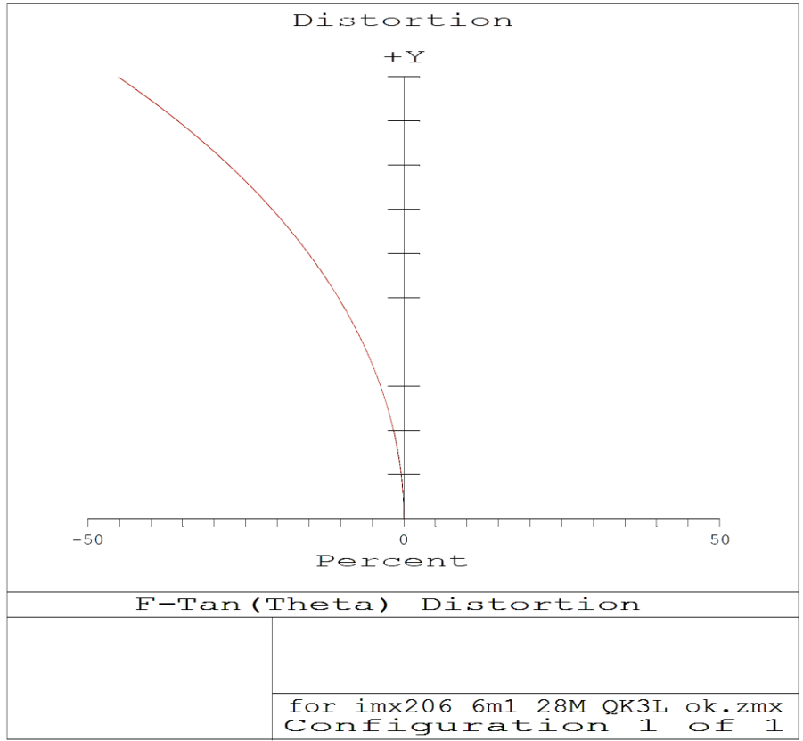
Figure 3: Optical Distortion
