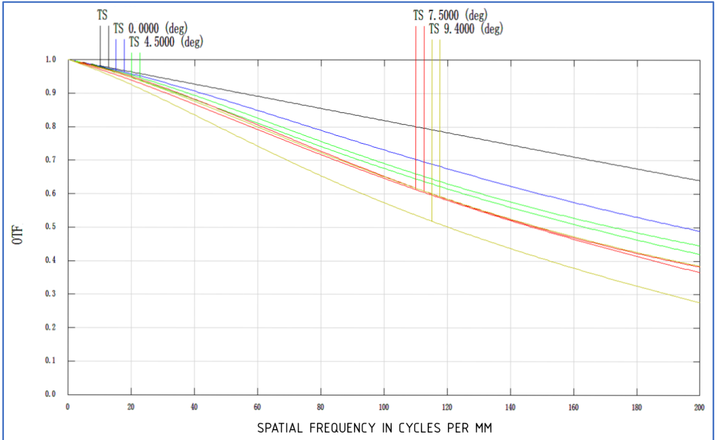
Figure 1: MTF Curves
