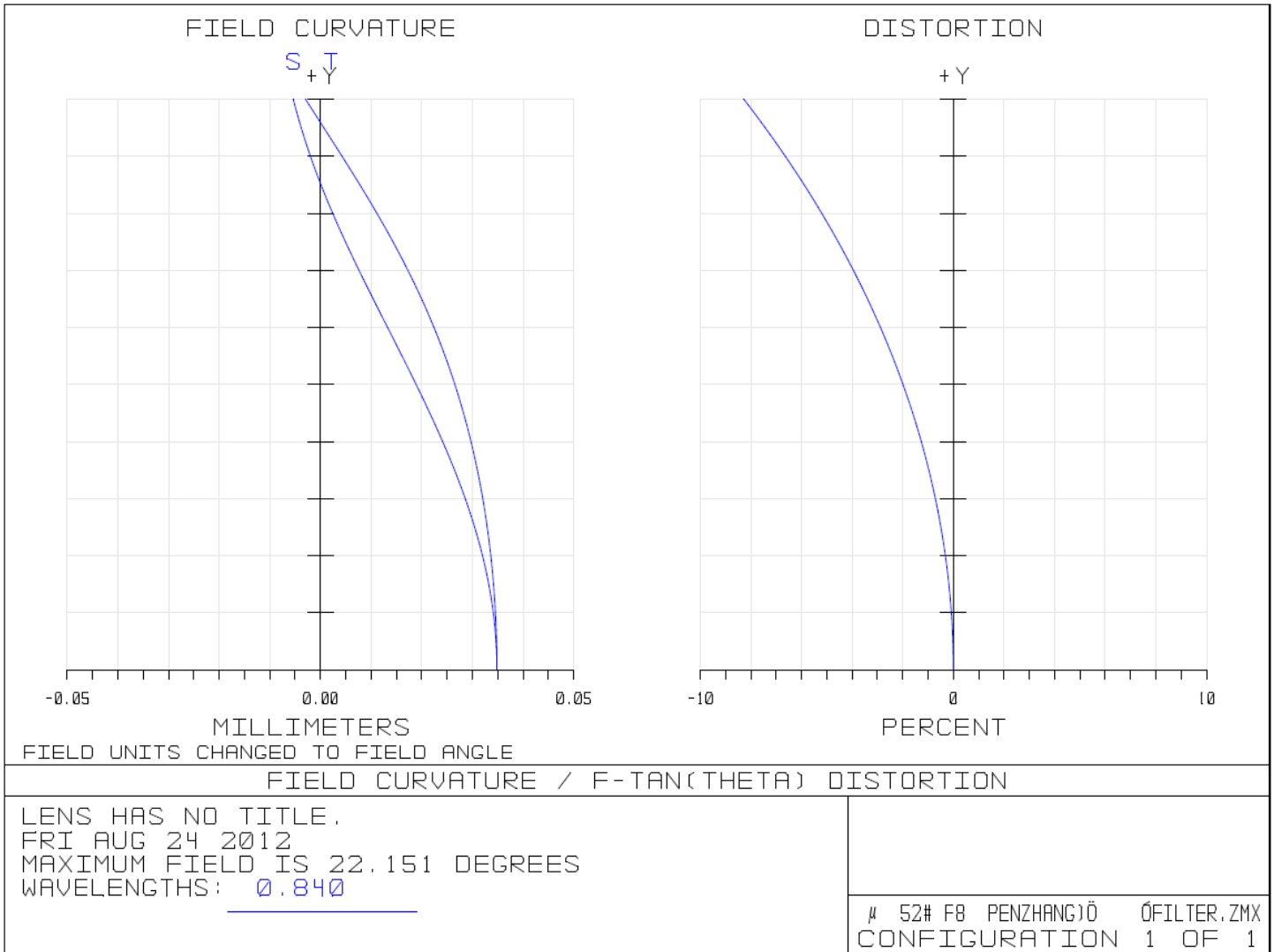
Figure 5: Field Curvature and Distortion (IR)
