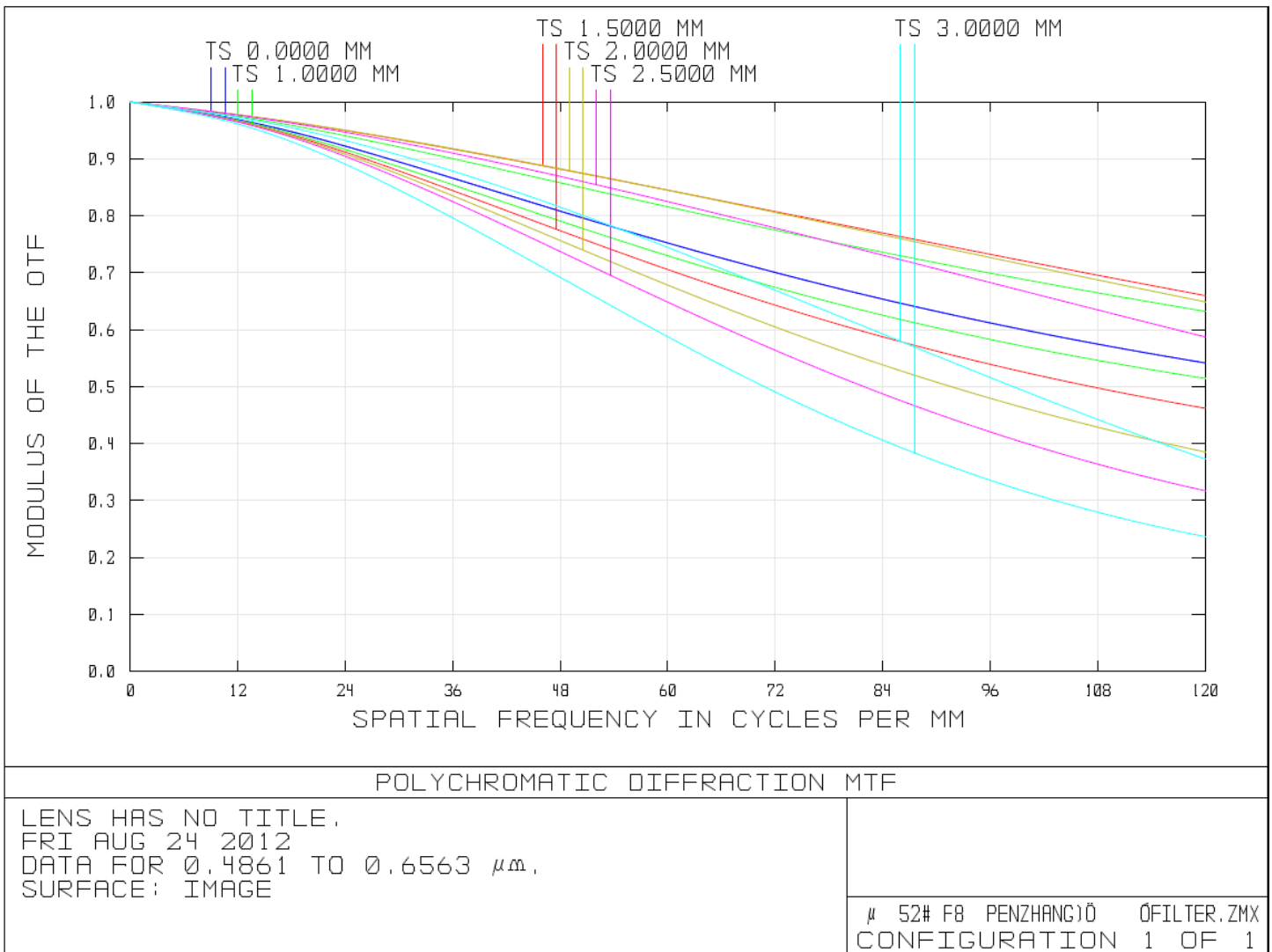
Figure 1: MTF Curves (Visible Light)
