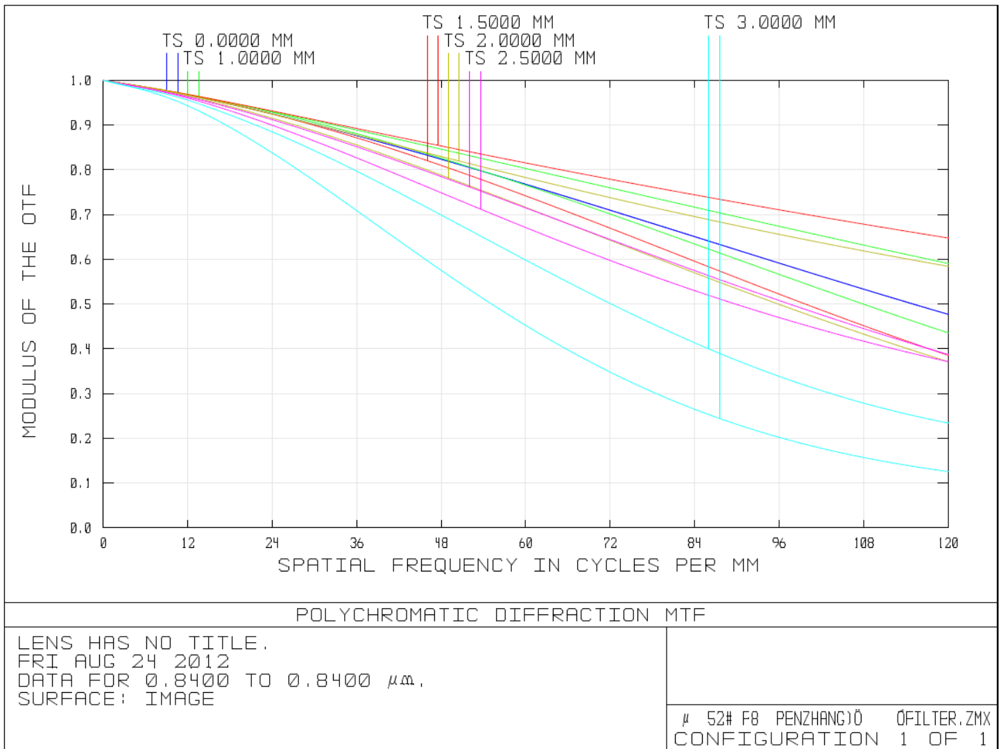
Figure 4: MTF Curves (IR)
