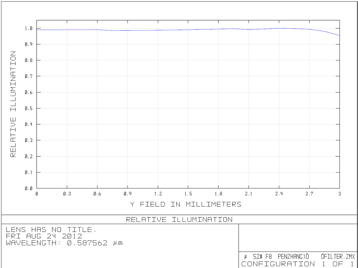
Figure 6: Relative Illumination (IR)
