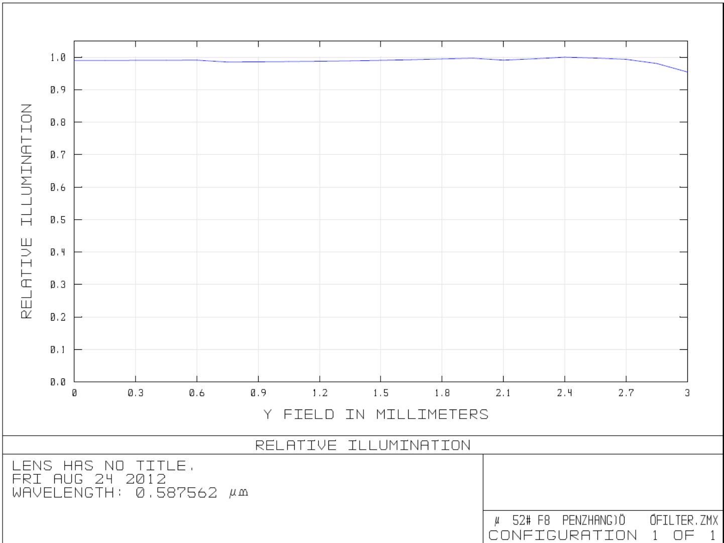
Figure 3: Relative Illumination (Visible Light)
