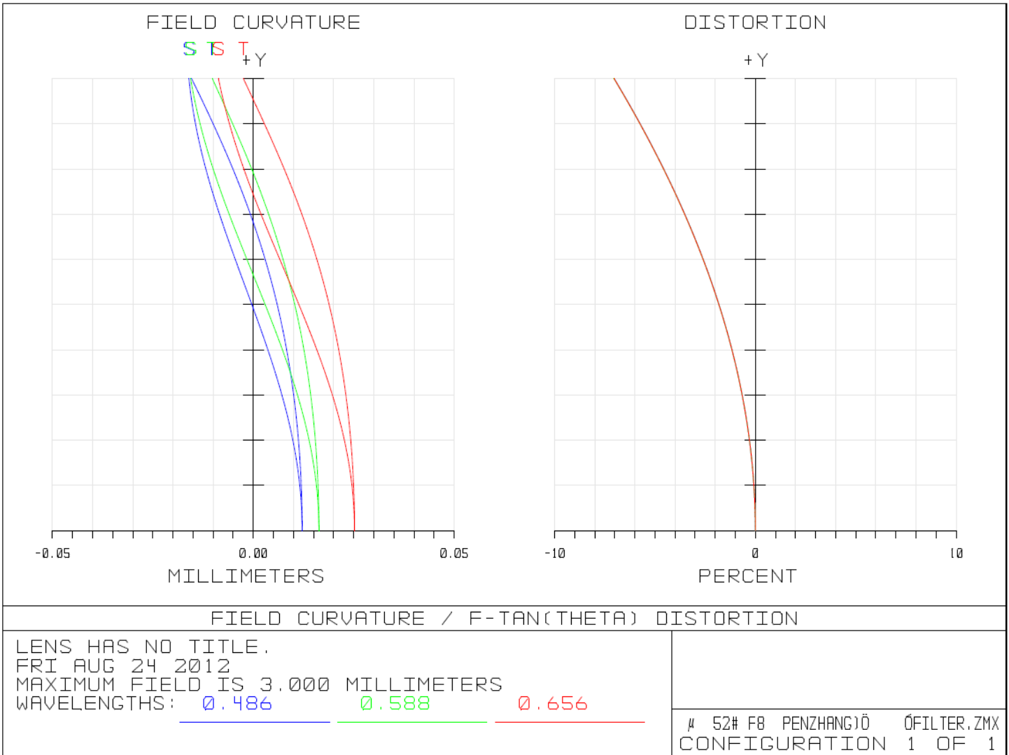
Figure 2: Field Curvature and Distortion (Visible Light)
