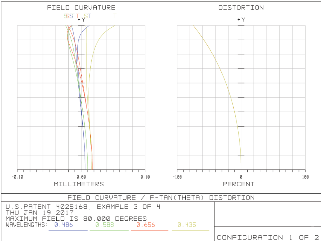
Figure 2: Field Curvature and Distortion
