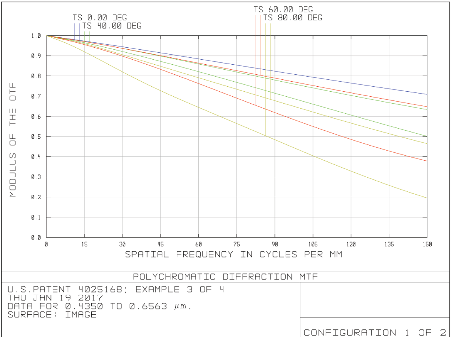
Figure 1: MTF Curves
