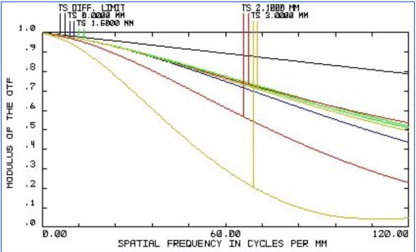
Figure 1: MTF Curves
