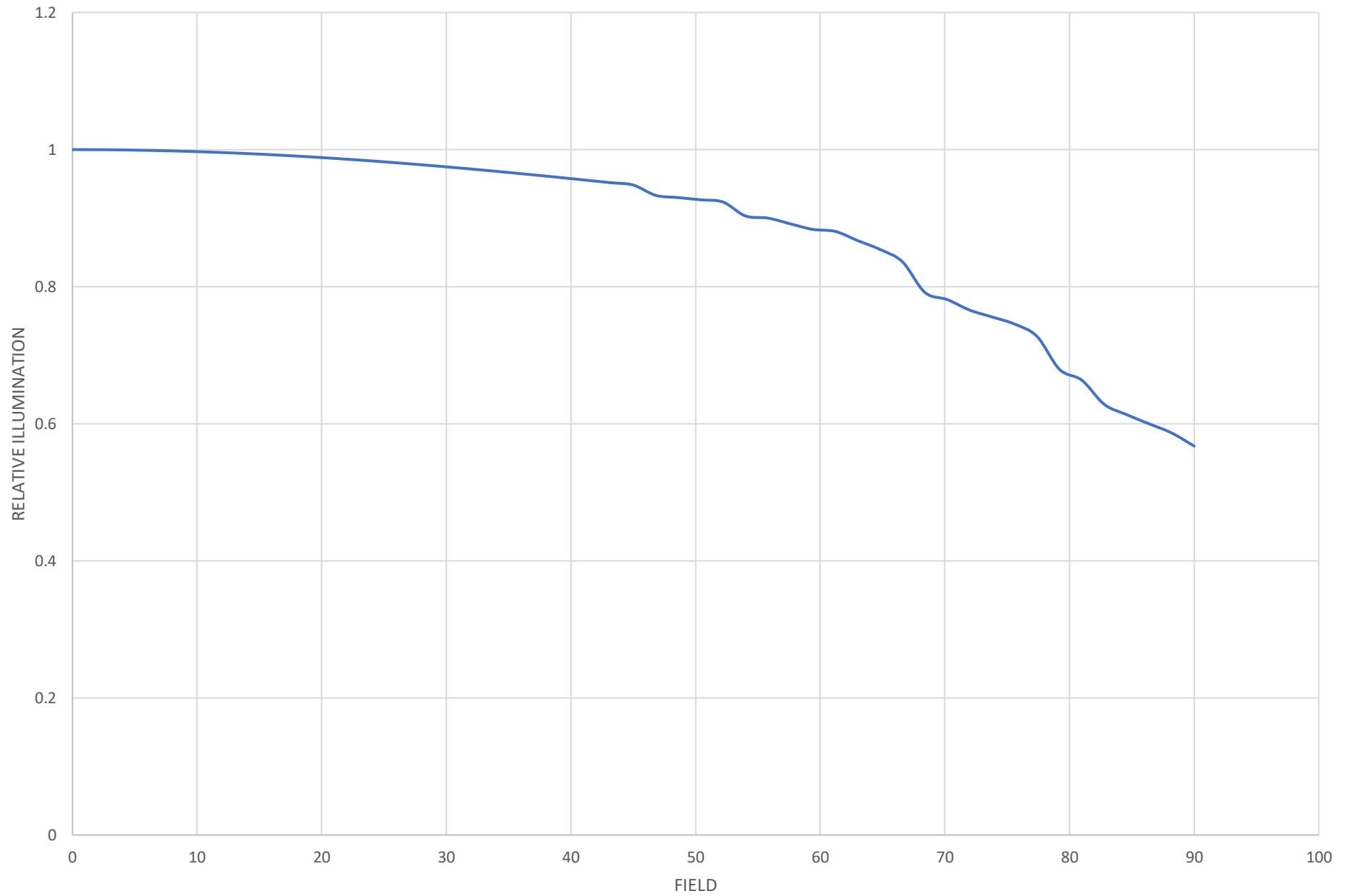
PT-017525XFL RELATIVE ILLUMINATION
