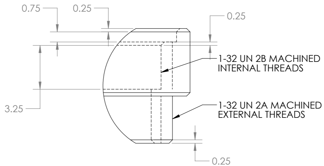
DETAIL A SCALE 6 : 1
